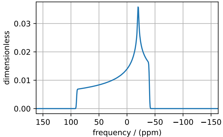
Solid-Echo Spectrum
