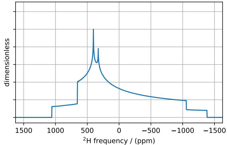
Half Single-Quantum Spectrum
