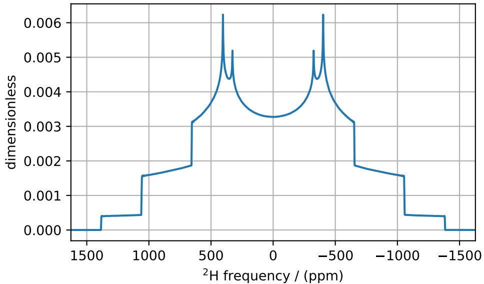
Full Single-Quantum Spectrum
