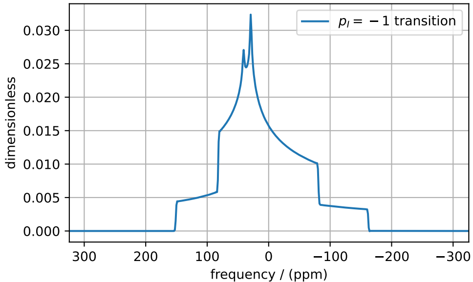
Single-Quantum Spectrum All Transitions
