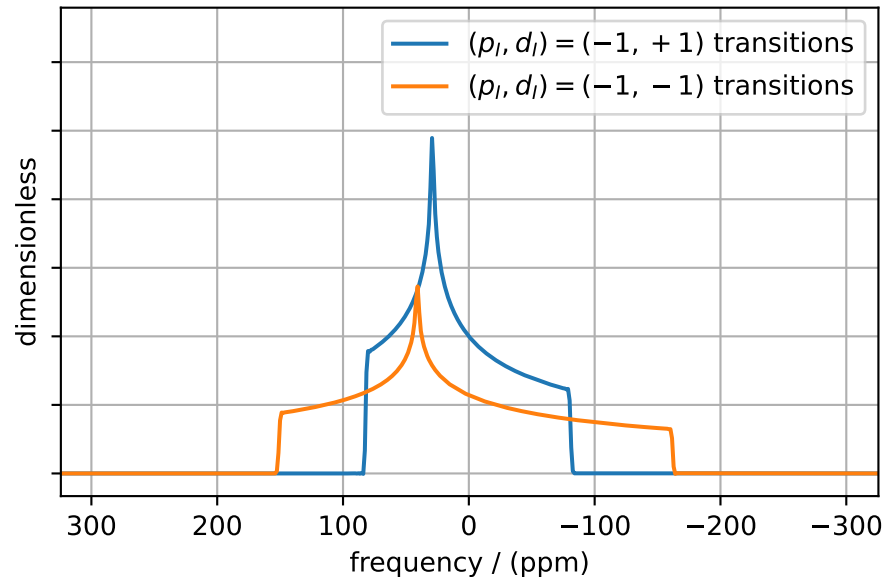
Single-Quantum Spectrum Single Transitions
