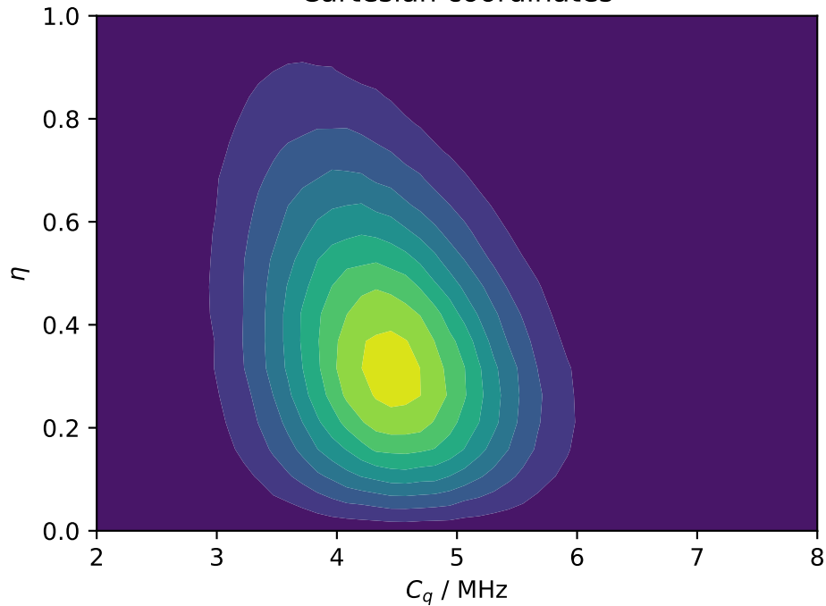
Cartesian coordinates
