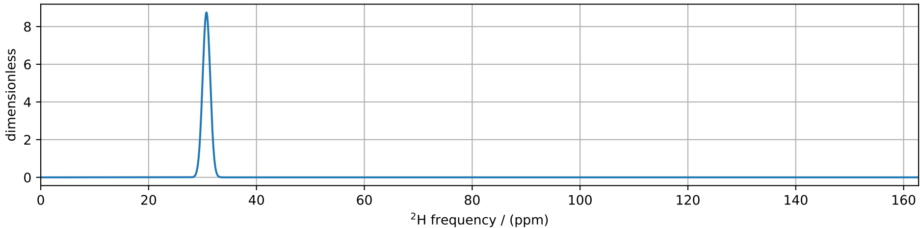
Heteronuclear Two-Spin ( ^2\text{H} - ^1\text{H} ) Triple-Quantum Spectrum
