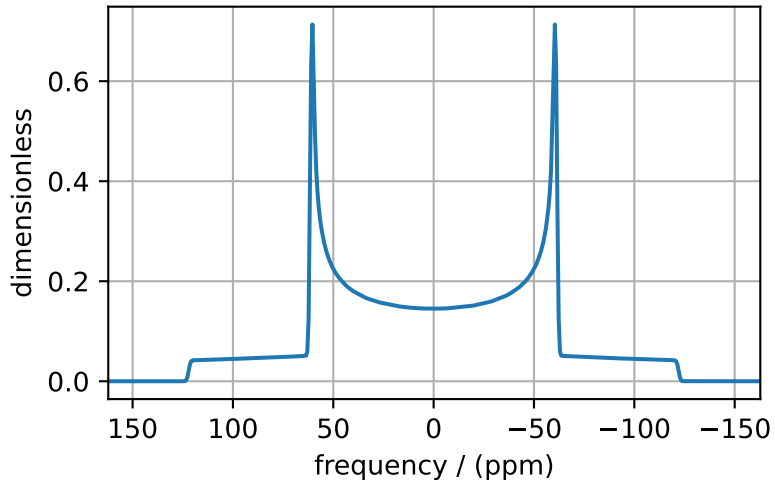
Hahn-Echo Spectrum
