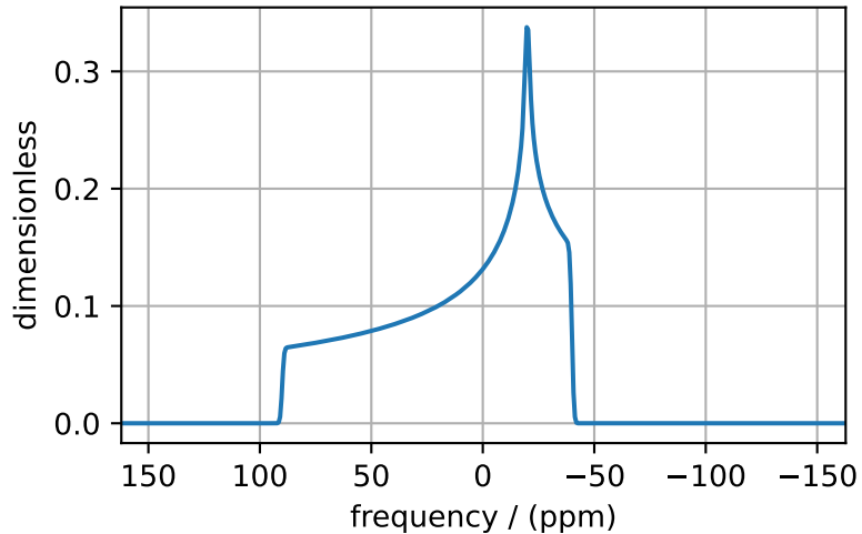
Solid-Echo Spectrum
