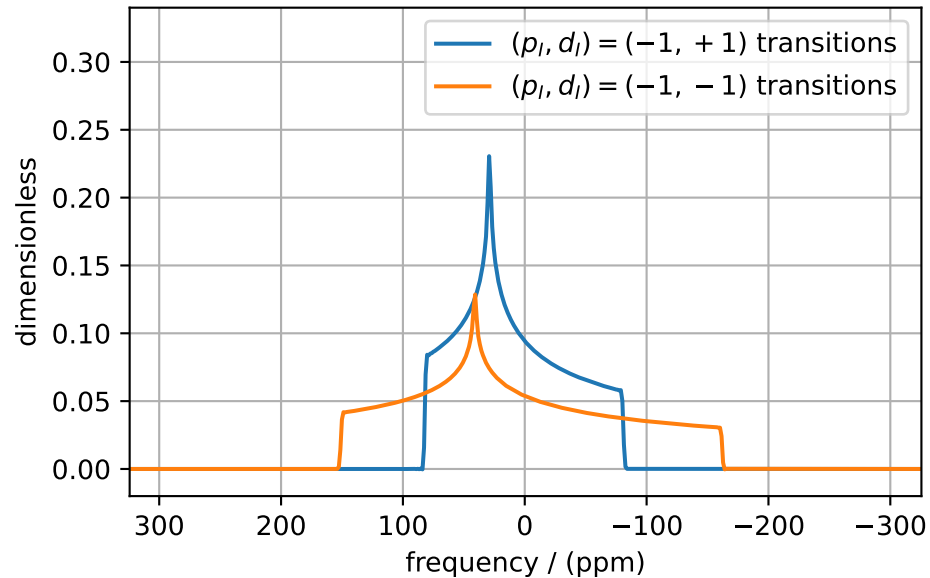
Single-Quantum Spectrum Single Transitions
