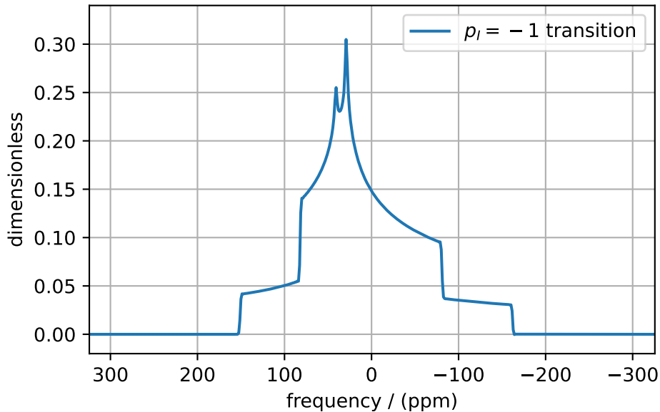
Single-Quantum Spectrum All Transitions
